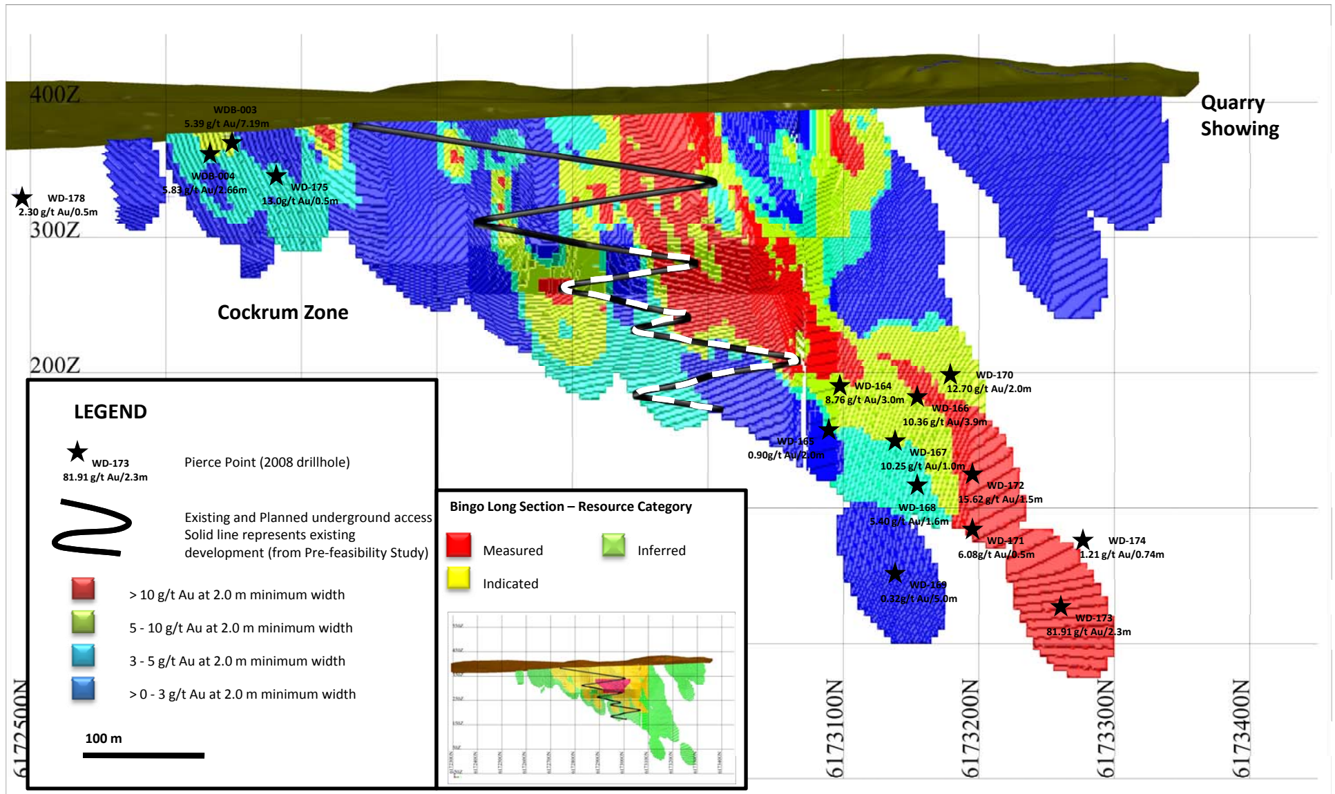
Figure 2: Bingo Gold Deposit – Longitudinal Section looking West
